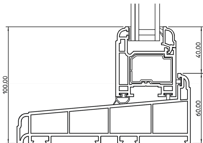
Bottom Rail
