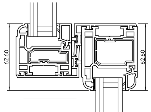
Meeting Rail
