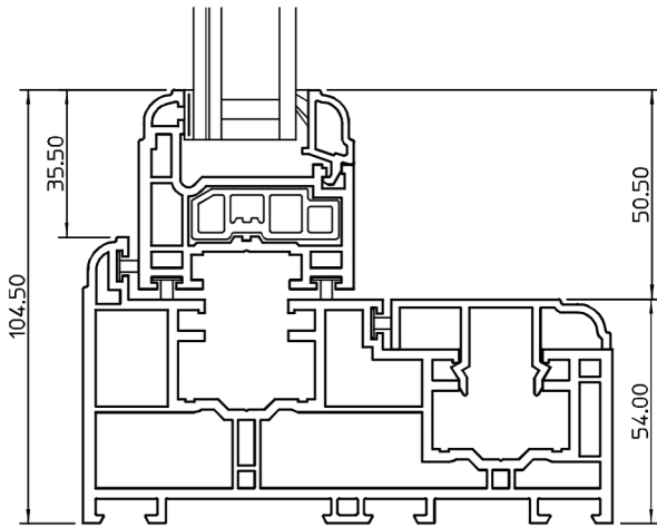
Top Rail
